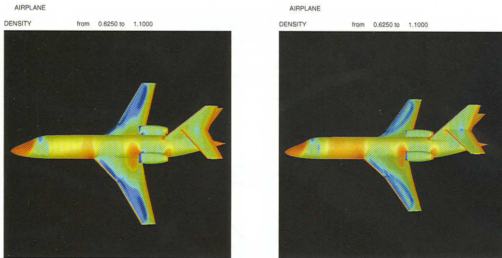
Figure 11. Comparison of density distributions on a Falcon before (left) and after (right) redesign.
