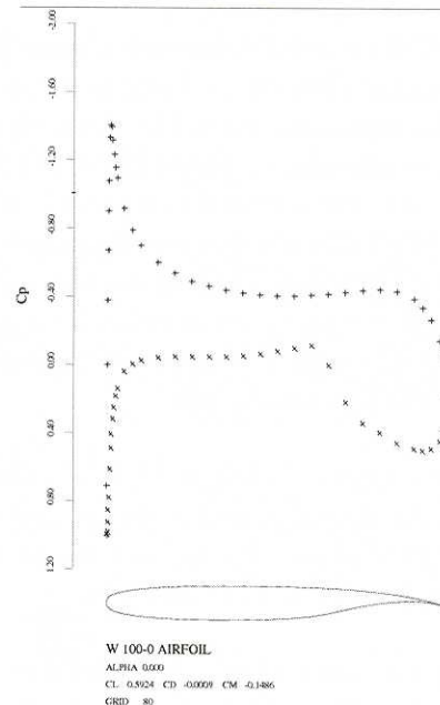
Figure 2. Inverse calculation, recovering the Whitcomb airfoil.
